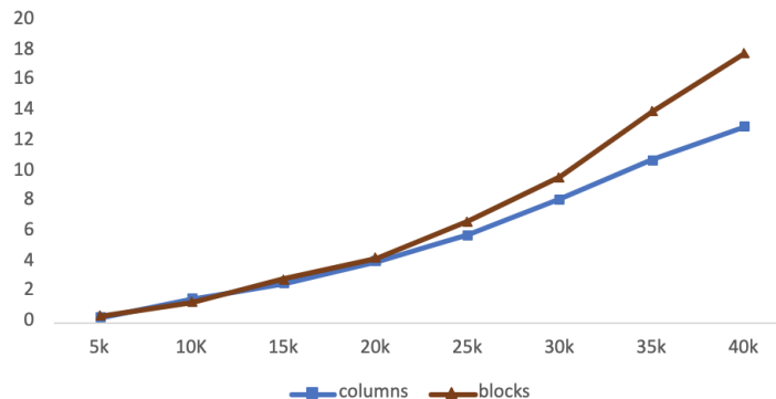
Figure 4: Weak scalability evaluation from 1 to 8 threads.
